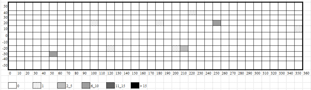
Synoptic map for the year 2010
