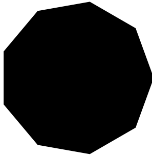
Regular polygon
