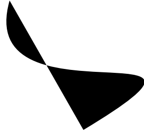
Bezier curve
